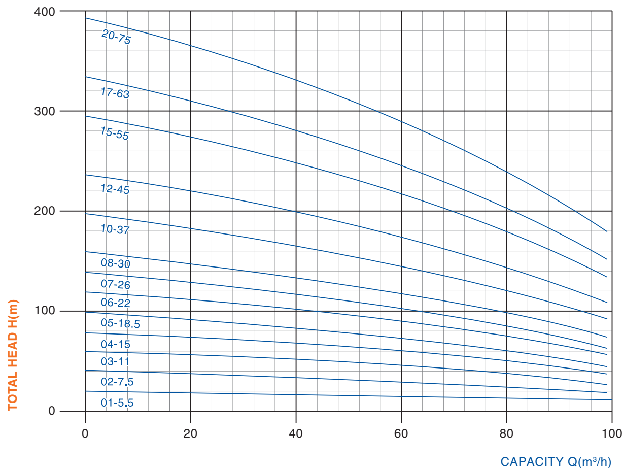
8SP77 SUBMERSIBLE PUMPS
