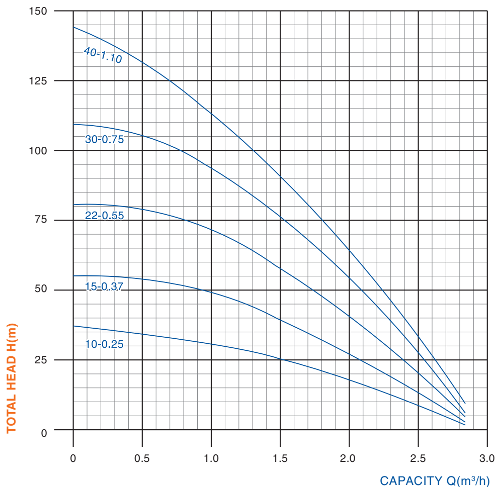
3SP1 SUBMERSIBLE PUMPS
